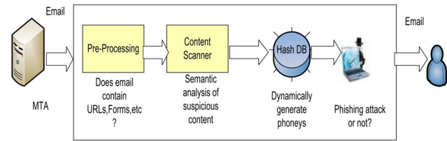
Fig. 16. Block diagram of PHONEY architecture [92]
