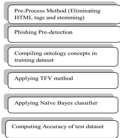
Fig. 15. Five steps in Ontology Concept proposed method [42].
